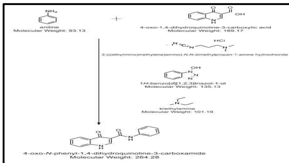
Fig.1- Reaction Scheme
